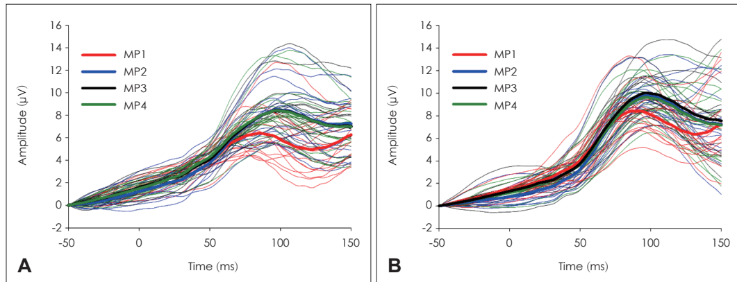
Supplementary Fig. 1. The individual cortical P1 onset responses in two groups. A: Non-musicians (n=15). B: Musicians (n=15). In the graph, the red line represents the auditory evoked potential (AEP) for the higher metrical position (MP1), while the other three lines correspond to the AEPs for the lower metrical positions (MP2, MP3, MP4).
